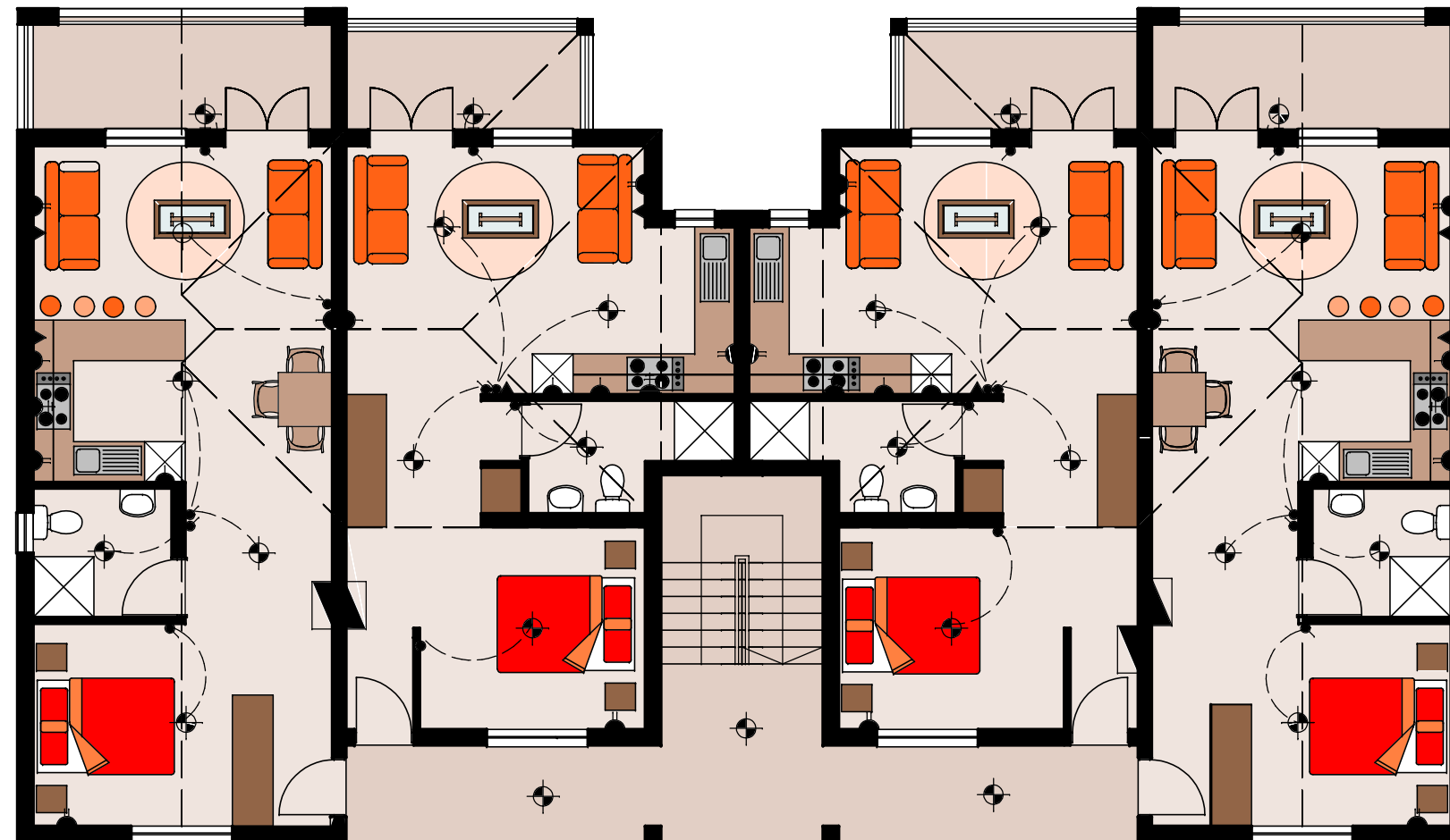
TYPICAL ONE BEDROOM UNIT LAYOUTS - 1:100
